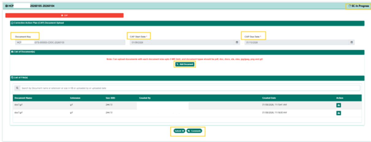
Figure 52: SC In-Progress
