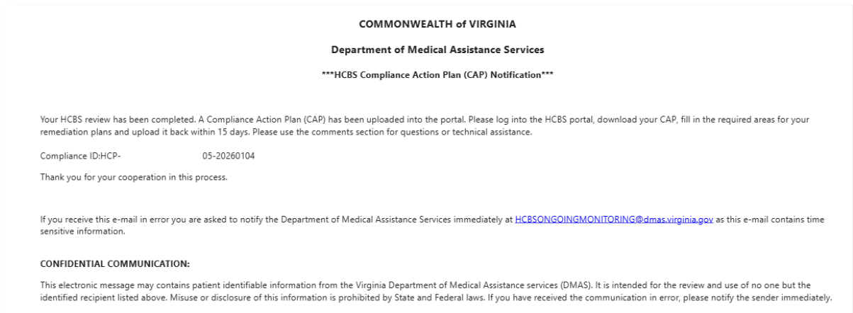
Figure 44: Provider Email
