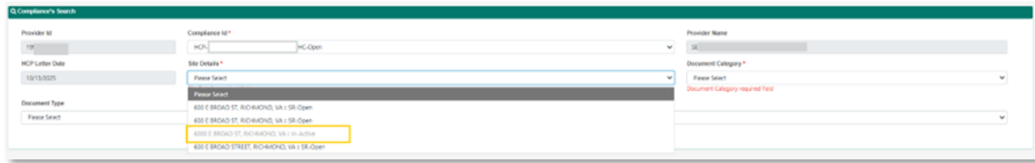
Figure 36: Inactive Indication
