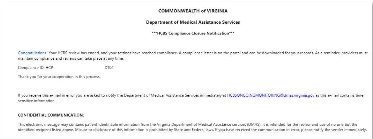
Figure 59: Email Notification
